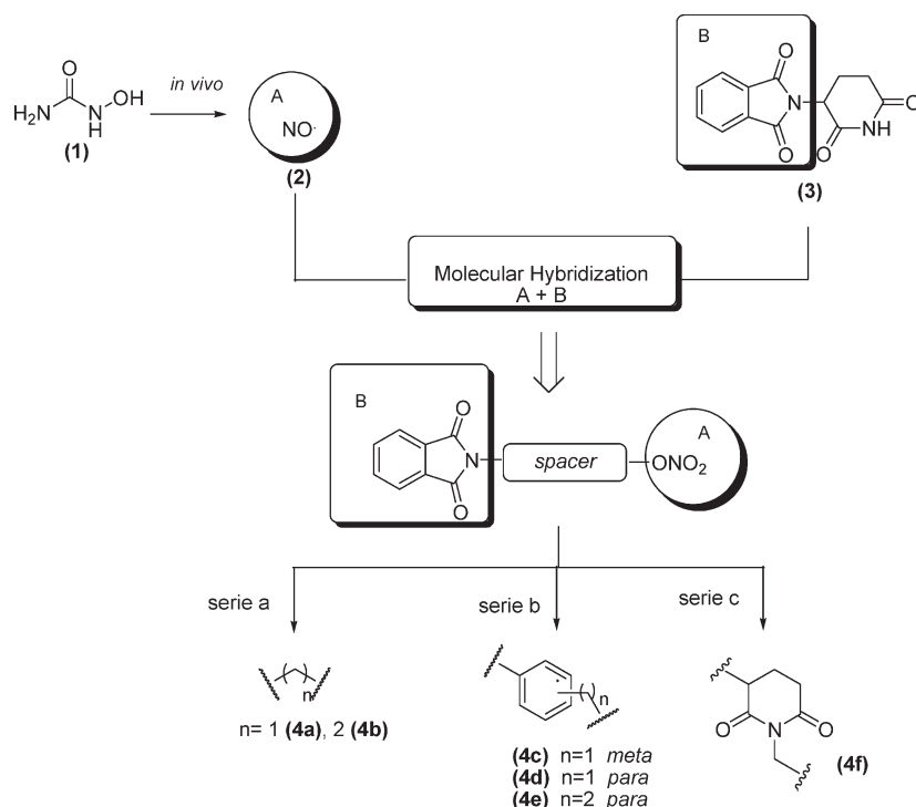
Scheme 1. Structural Planning Using Molecular Hybridization
